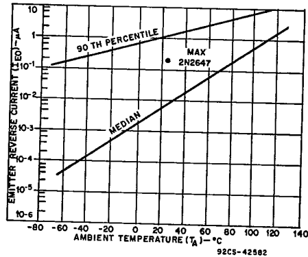
Fig. 7—Typical emitter reverse current characteristics.
