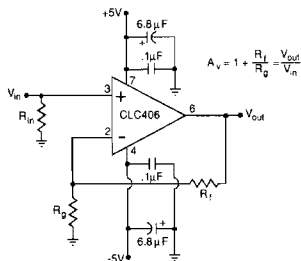
Figure 1: recommended non-inverting gain circuit
