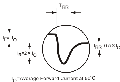
TYPICAL REVERSE RECOVERY WAVEFORM
