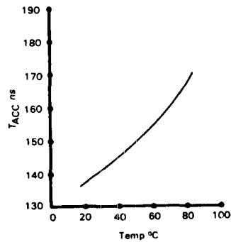
Typical T ACC vs Temp
