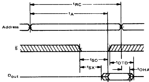
READ CYCLE TIMING (Note 5)
