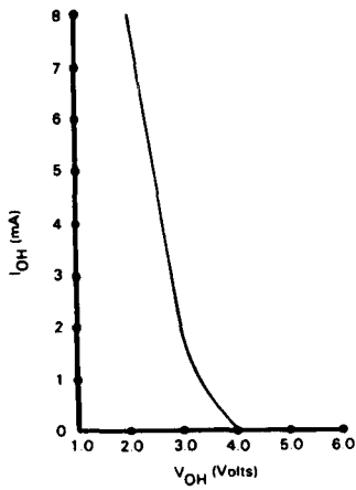
Output Source Current vs Output Voltage
