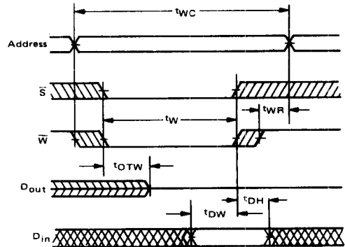
WRITE CYCLE TIMING (Note 6)
