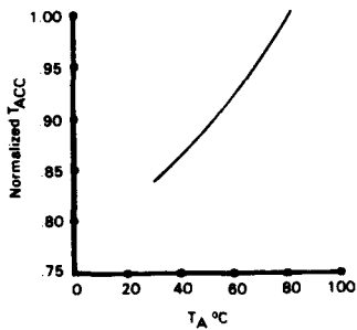
Normalized T ACC vs Temperature
